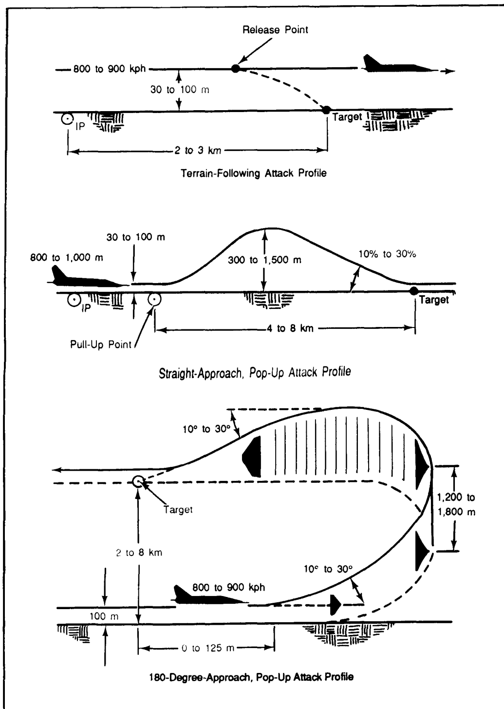
Figure 7-2. Typical Aerial Attack Profiles Against Fixed Facilities
